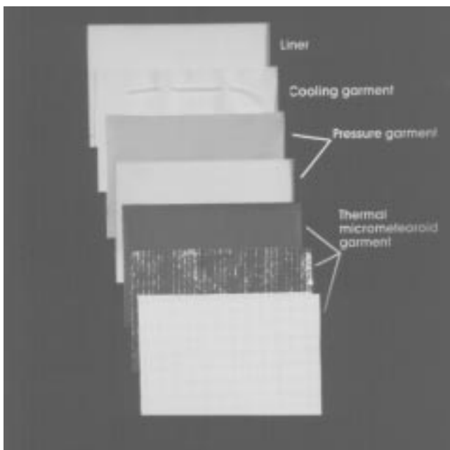
Each layer of a space suit has a purpose. Many thin layers also make the suit more resistant to micrometeoroid penetration than a single, thick layer would be.
