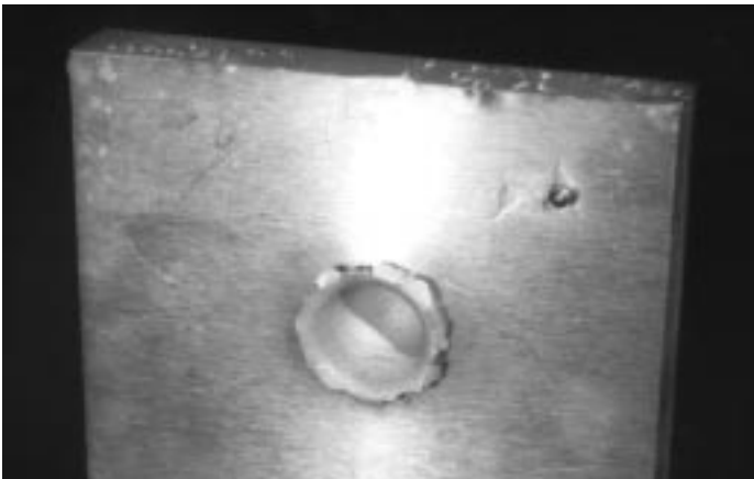
This block of aluminum shows the damage caused by a BB-sized object moving about 6,000 m/s (13,400 mph), which is slower than orbiting objects move. (Crater shown actual size.)
