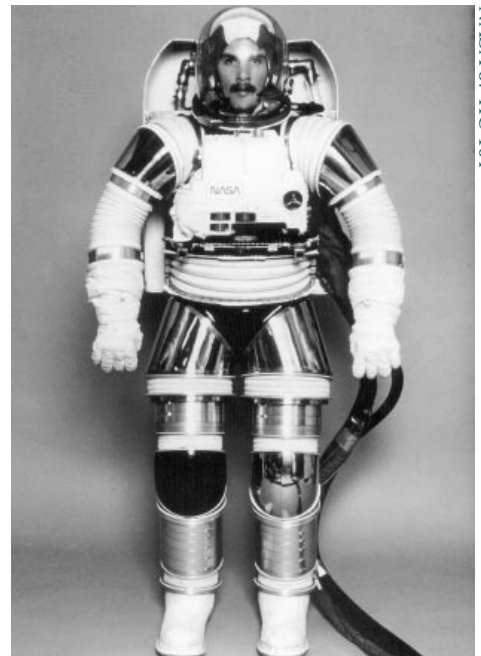
The next generation of space suits will probably be rigid. Unlike soft suits, hard space suits can maintain standard sea-level pressure.
