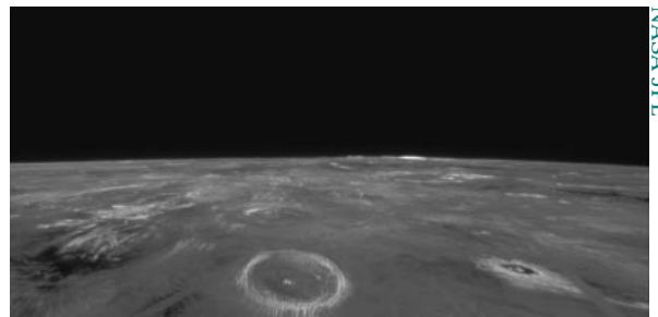
Three-dimensional images were constructed from Magellan data for the fly-over sequences in the film. Magellan ’s radar peered through the dense atmosphere of Venus to map the surface. (Note: Only the surface is shown, the Venus’ “sky” is not dark during the day.)
